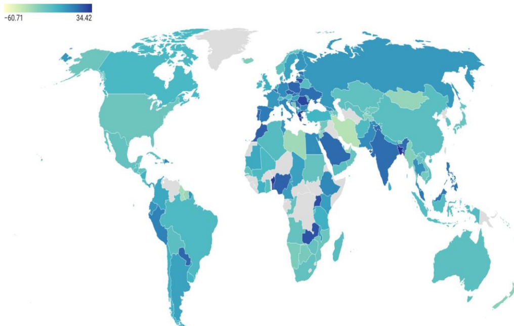
Fig. 6. Development Index.
